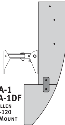
ALA-1LT, ALA-1 & ALA-1DF w/ALLEN MM-120 MULTIMOUNT
