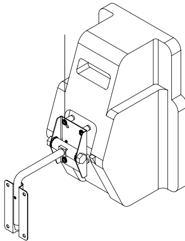
EON10-KT with MM-022 Wall Mount (Horizontal installation-arm down)
