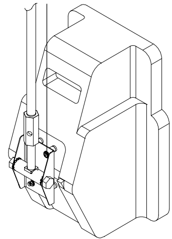
EON10-KT with MM-022 Wall Mount (Horizontal installation-arm down)
