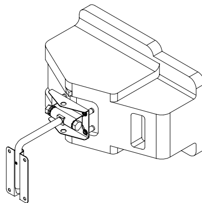
EON10-KT with MM-022 Wall Mount (Horizontal installation-arm down)
