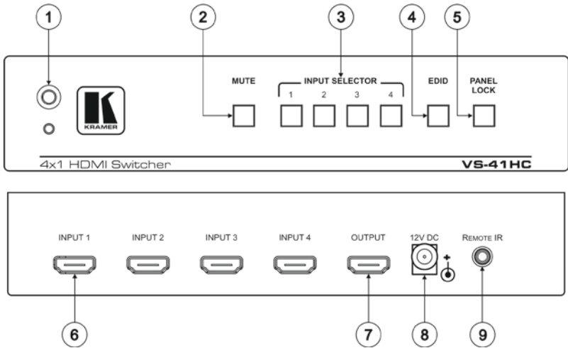
Figure 1: VS-41HC 4x1 HDMI Switcher
