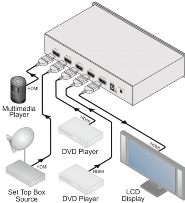
Figure 2: Connecting the VS-41HC 4x1 HDMI Switcher
