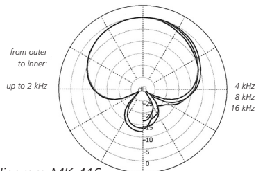
Polar diagram MK 41S
