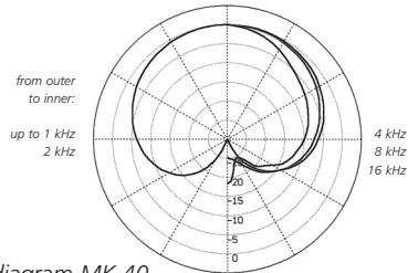
Polar diagram MK 40
