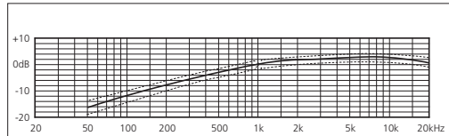
Frequency response curve MK 4A + CMC 6
