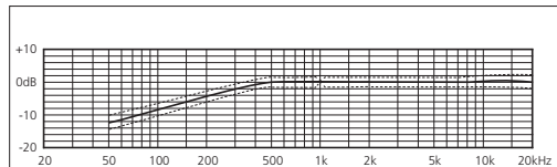
Frequency response curve MK 41S + CMC 6
