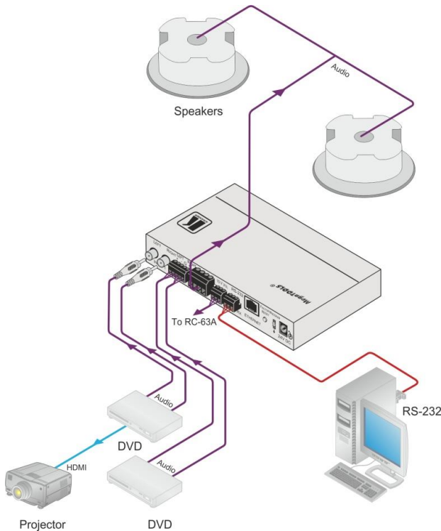
Figure 1: Yarden 4-C Closed-back Ceiling Speaker in a Boardroom Setup
