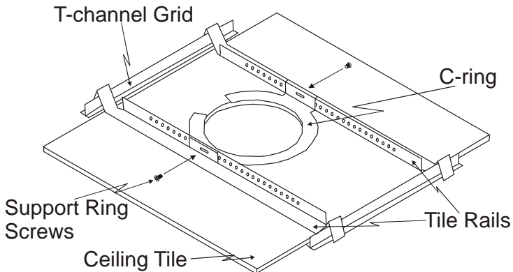
Figure 4: Mounting the Yarden 4-C Closed-back Ceiling Speaker
