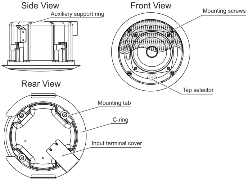
Figure 2: Yarden 4-C Closed-back Ceiling Speaker
