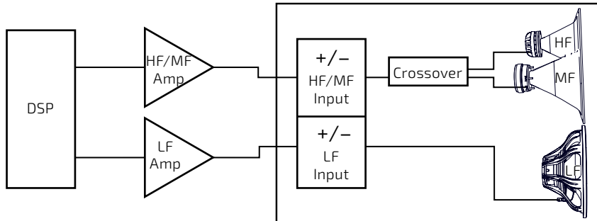
Three-way biamp
