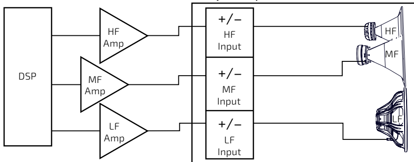
Three-way triamp
