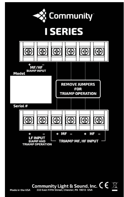
Three-way input panel
