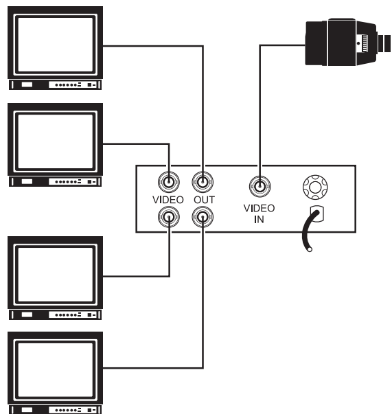
TYPICAL CONFIGURATION
