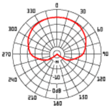
AMPLITUDE VS. ANGLE 1 KHz
