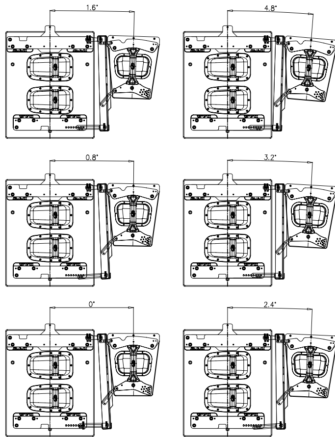
Splay angles using the AX-Combo12, aero 12A and LX-218RA.
