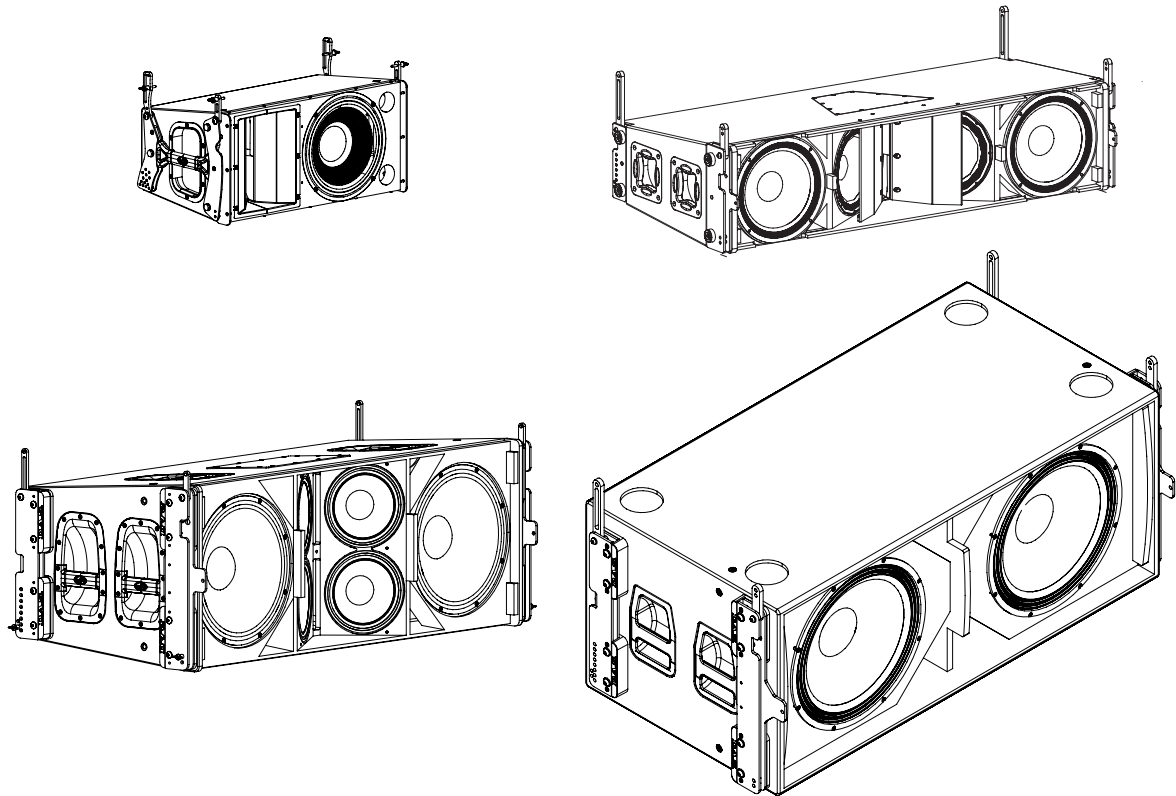
Diagram of the guides in the rigging hardware of the aero 12A , aero 38 , aero 38A , aero 50 , LX-218R and LX-218RA .
