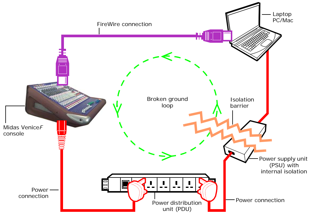
Isolated FireWire computer system. Note how the isolation barrier breaks the ground loop.
