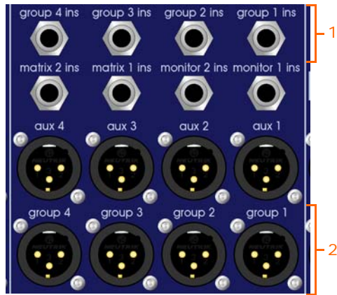
Group connectors on rear panel
