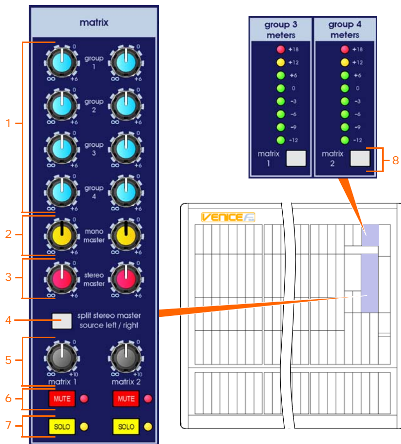
matrix output section on the control surface
