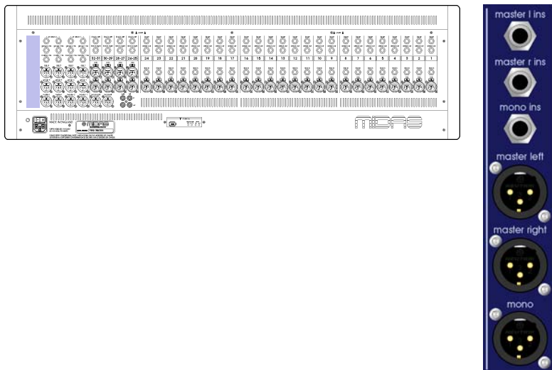
Master outputs on the rear panel
