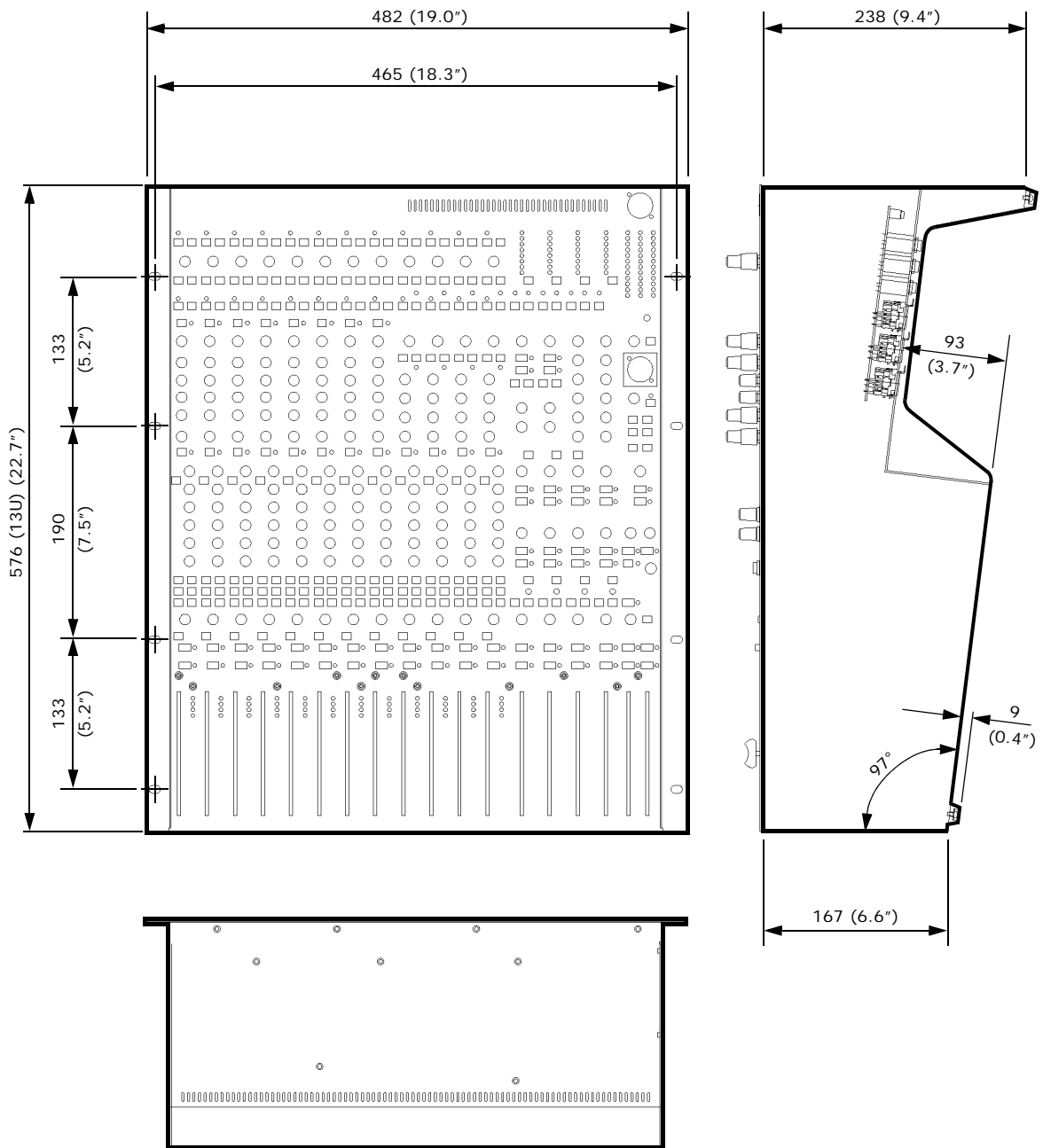
External dimensions of the F16R rack mount console
