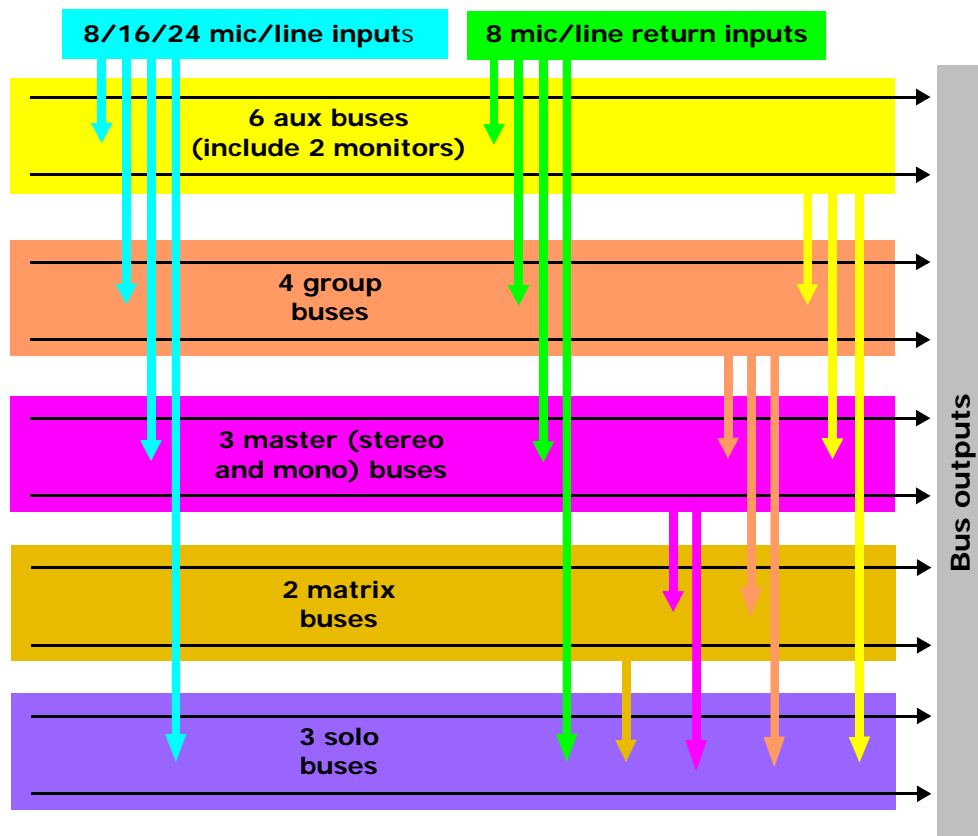
VeniceF mix matrix
