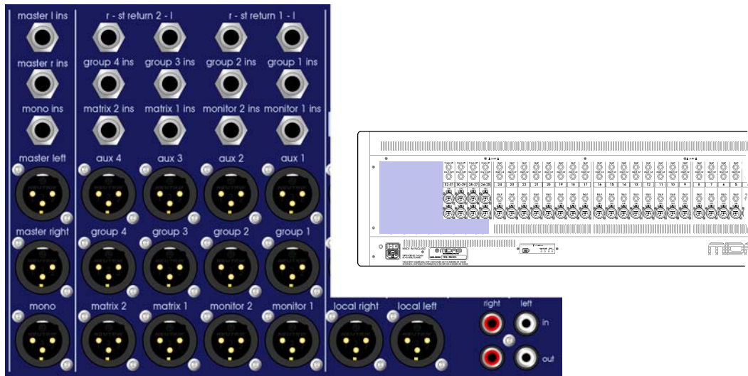
Output connections on rear panel
