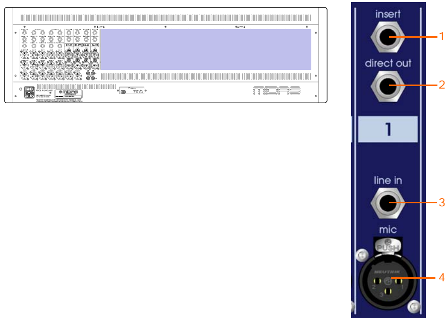
Mono input channel connectors
