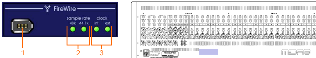
FireWire section on the rear panel
