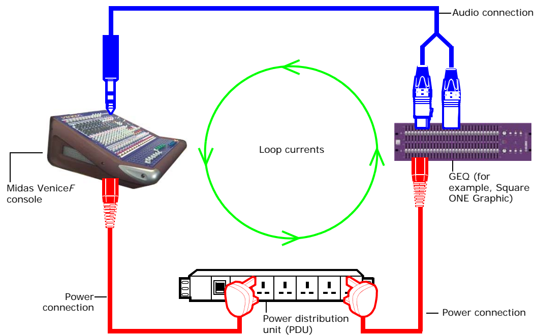
Ground loop
