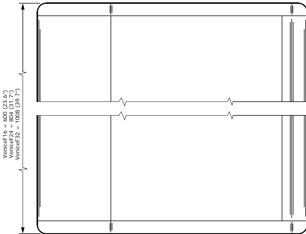
External dimensions of the F16, F24 and F32 consoles
