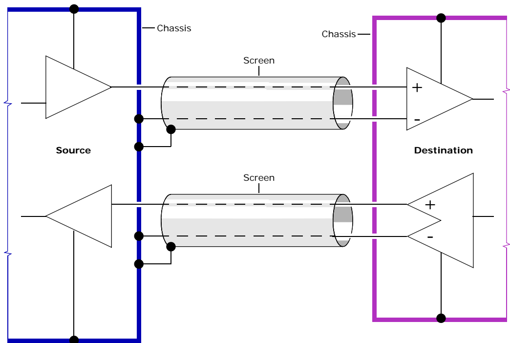
Ground referenced insert wiring diagram. For a typical example of how to wire a ground referenced insert, see Figure 1 on page 13; the example above shows the screen connection at the other end because it is more practical, as it reduces the wiring complexity within the 1/4" TRS Jack connector.
