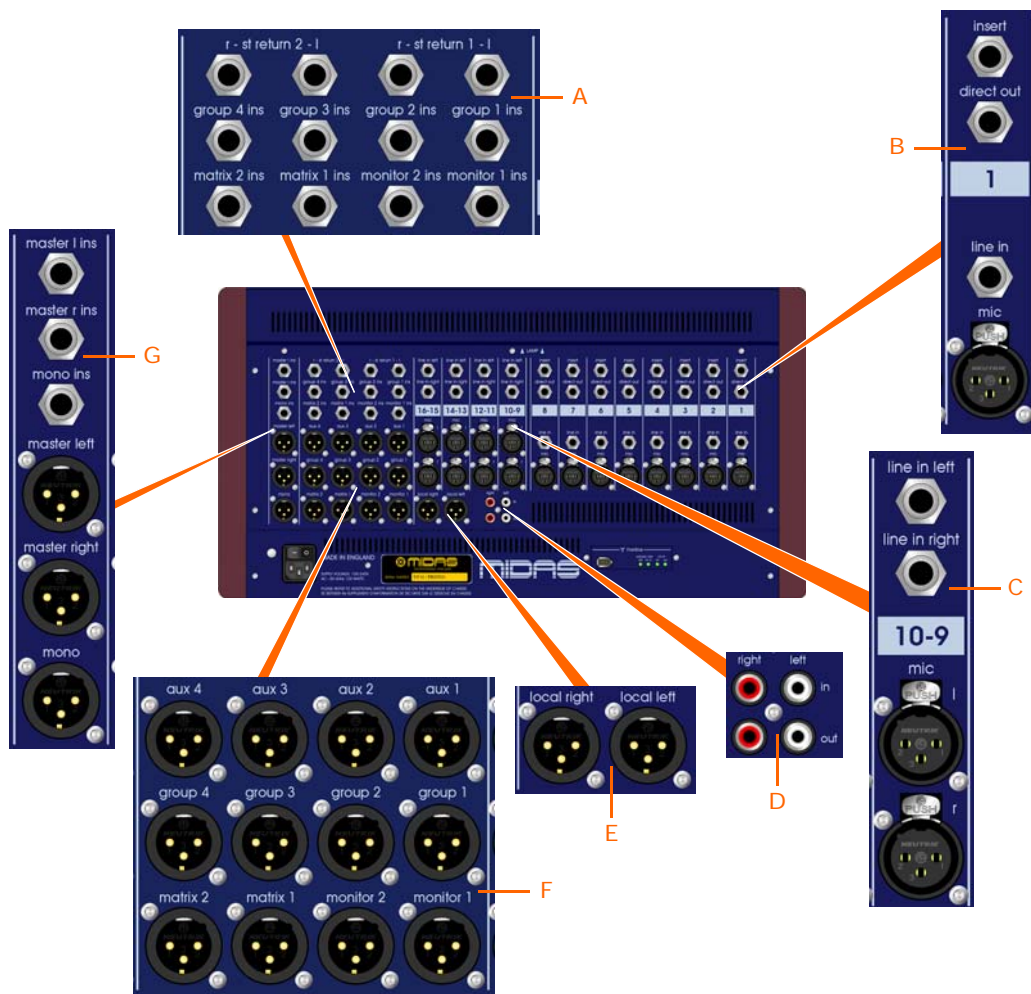
Rear panel of the VeniceF16 showing the main connector sections
