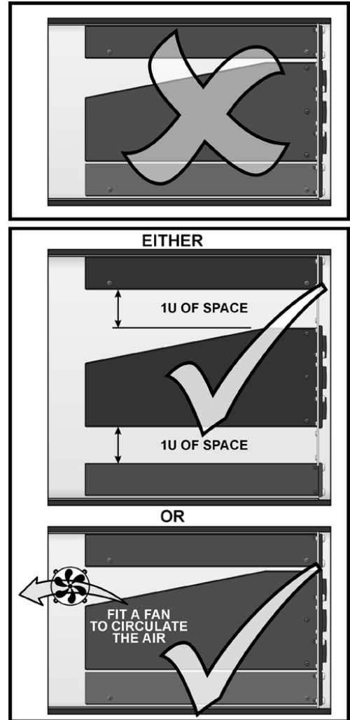
fig.1 RACK MOUNT POSITIONING
