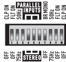
Typical Mode Switch block as seen from the rear of the amplifier (CX404V model shown).
