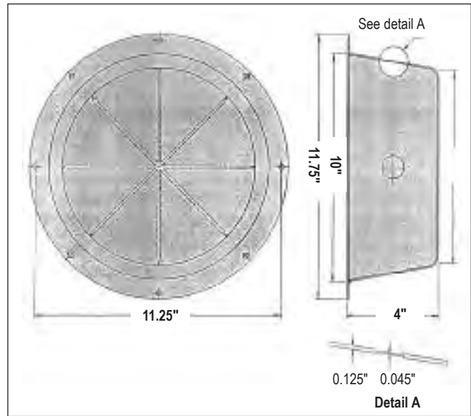
Dimensions for Model 8SPBX
