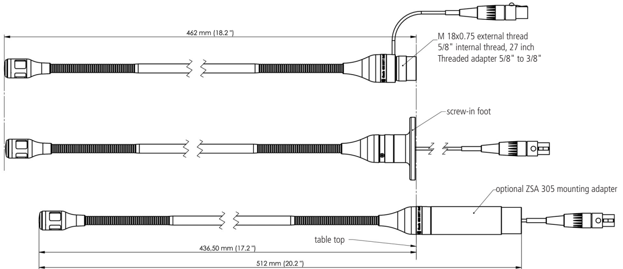
ZSH 305 screw-in foot
