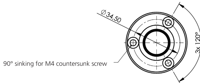
ZSH 305 screw-in foot
