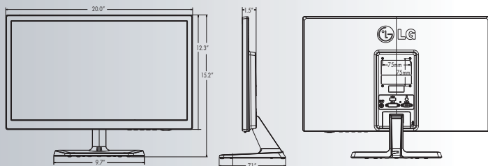
IPS224V-PN
