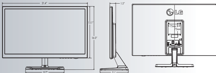
IPS234V-PN
