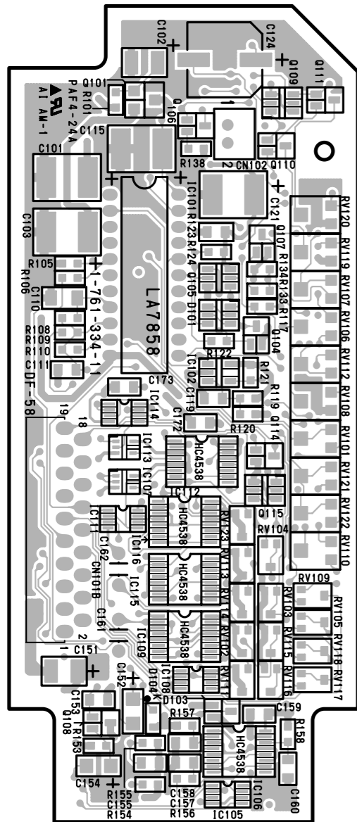
DF-58 -COMPONENT SIDE- SUFFIX: -11
