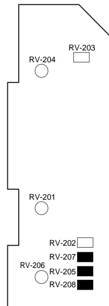
VR-266 - component side -
