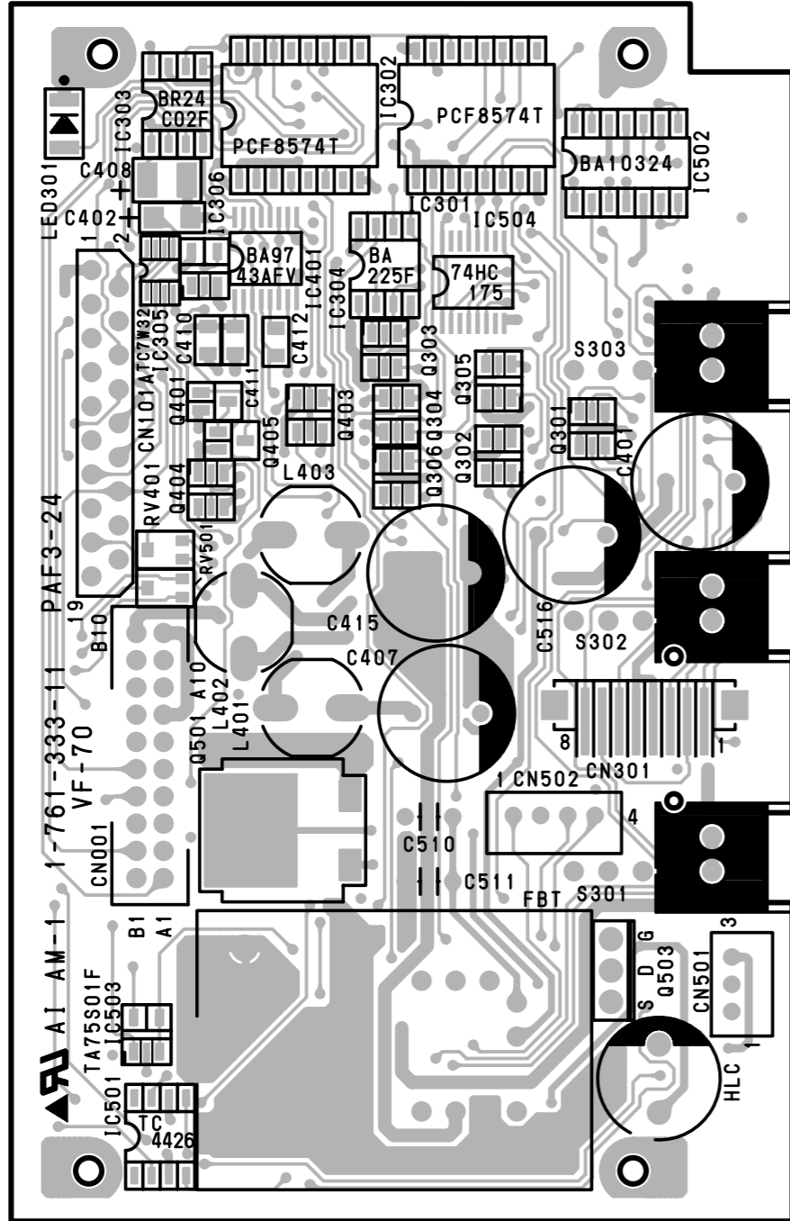
VF-70 -COMPONENT SIDE- SUFFIX: -11
