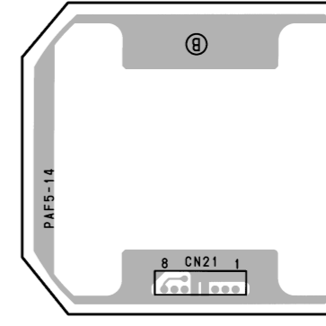
LP-105 -B SIDE- SUFFIX: -11
