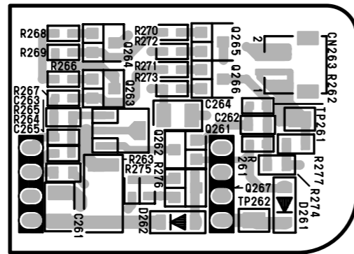
VDA-41 -SOLDERING SIDE- SUFFIX: -11
