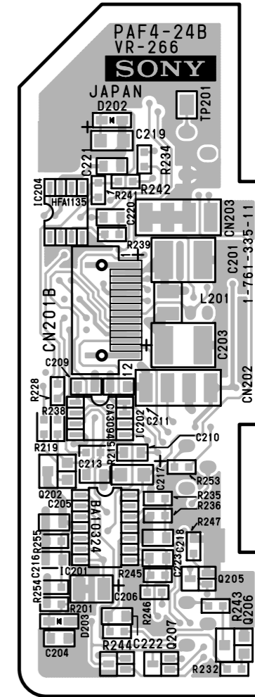
VR-266 -SOLDERING SIDE- SUFFIX: -11
