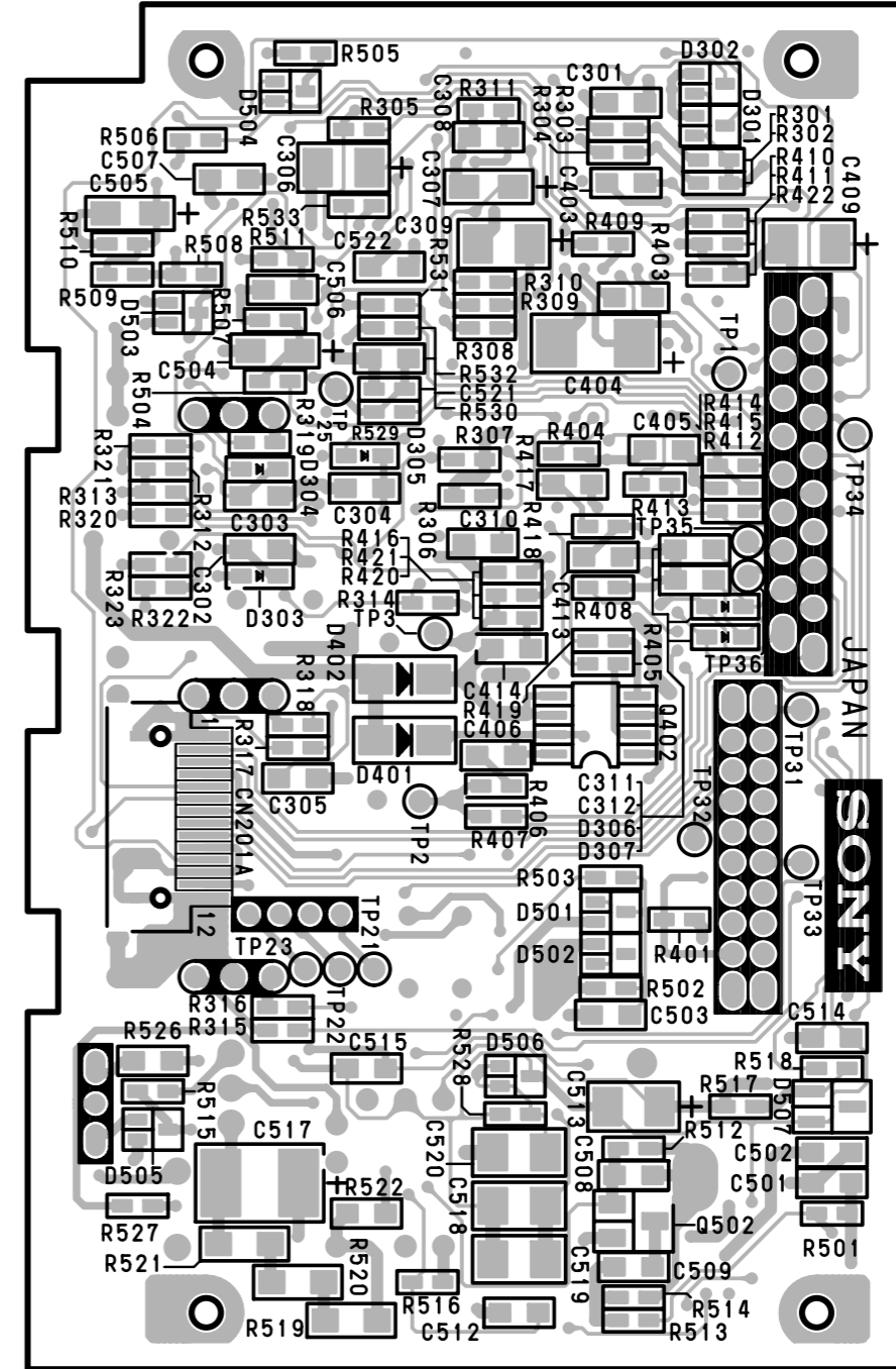
VF-70 -SOLDERING SIDE- SUFFIX: -11
