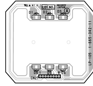
LP-105 -A SIDE- SUFFIX: -11
