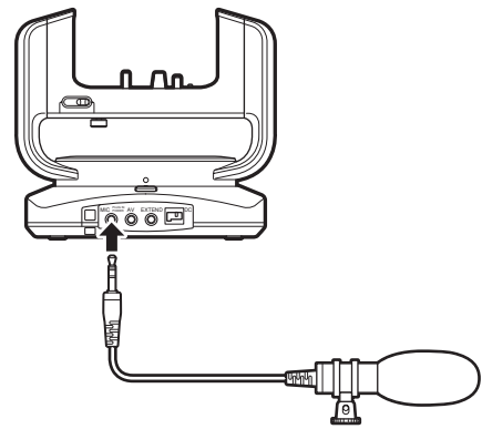
Mic (commercially available) φ3.5 mm stereo mic jack
