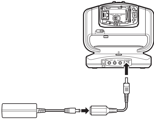
AC adapter (supplied) Conversion cable (supplied)
