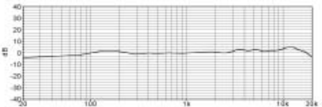
NT1-A Frequency Response
