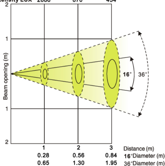
Beam angle 16° Field angle 36° of Red LEDs ( LENS 25° ) Intensity LUX 2686 870 434
