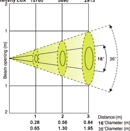
Beam angle 16° Field angle 36° of Full LEDs ( LENS 25° ) Intensity LUX 15760 5890 2913
