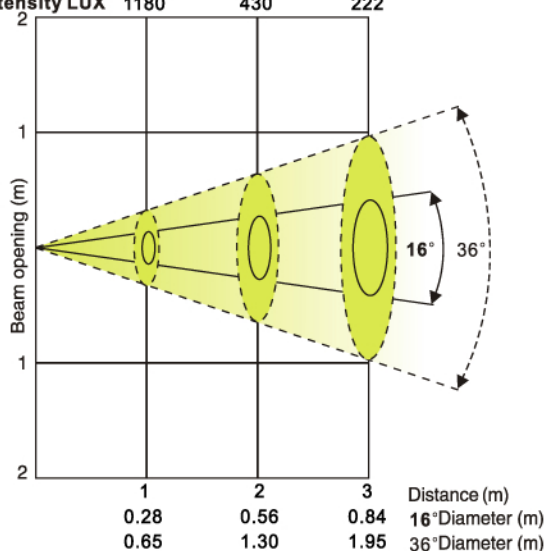
Beam angle 16° Field angle 36° of Blue LEDs ( LENS 25° ) Intensity LUX 1180 430 222
