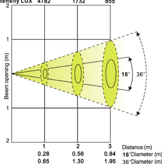
Beam angle 16° Field angle 36° of White LEDs ( LENS 25° ) Intensity LUX 4782 1732 855
