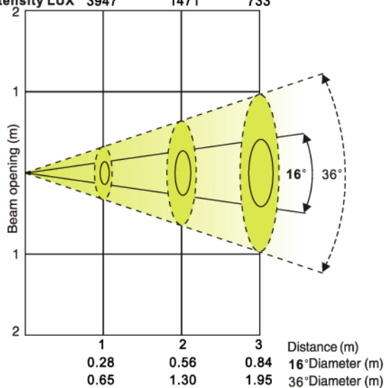
Beam angle 16° Field angle 36° of Amber LEDs ( LENS 25° ) Intensity LUX 3947 1471 733
