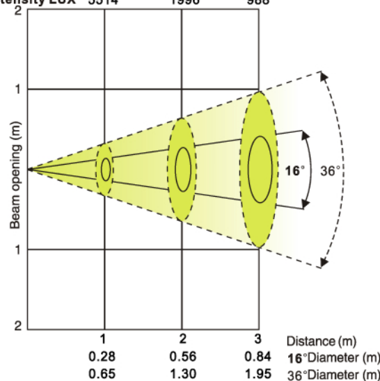
Beam angle 16° Field angle 36° of Green LEDs ( LENS 25° ) Intensity LUX 5514 1996 988
