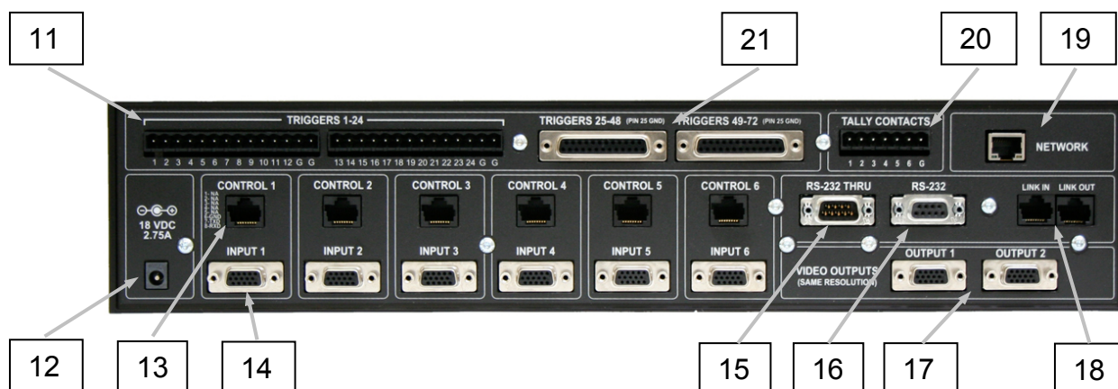
ControlVIEW XHD Back Panel I/O (Figure 3):
