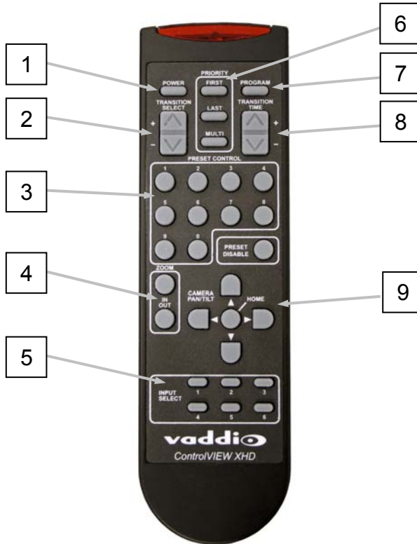
Figure 4: ControlVIEW XHD IR Remote Control
