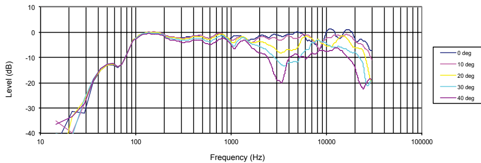
LOWER VERTICAL OFF-AXIS RESPONSE
