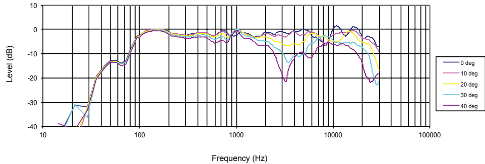
UPPER VERTICAL OFF-AXIS RESPONSE
