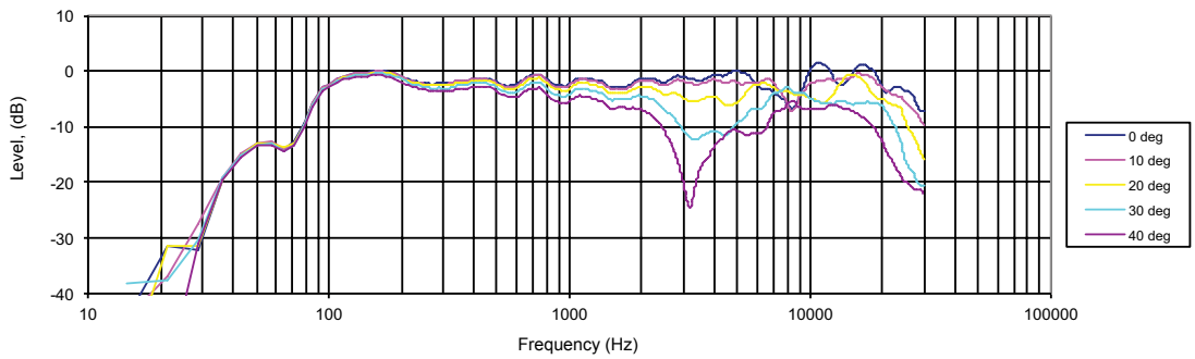
Horizontal Off-axis Frequency Response
