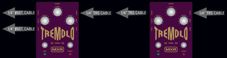
TRS Stereo In to Discrete Stereo Out
