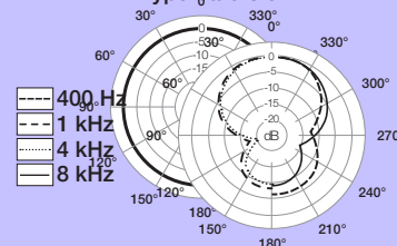
1 kHz Polar Response measured at 6 inches hypercardioid
