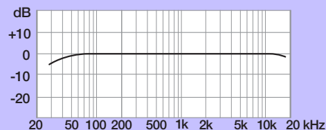
Frequency Response omni, measured at 6 inches
