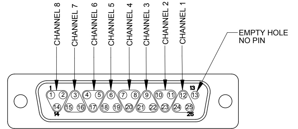
DB25 PIN-OUT VIEW
