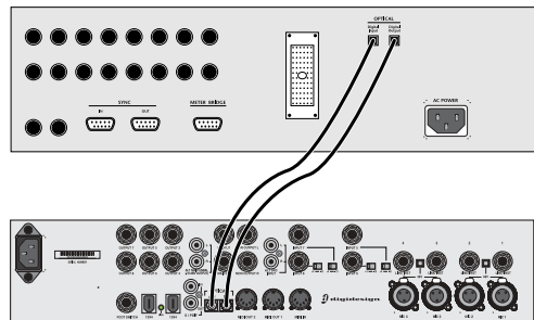
Connecting an ADAT to Digi 002 Rack
