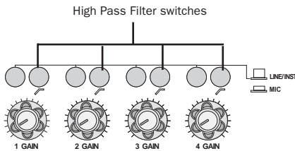
High Pass Filter switches (front panel)
