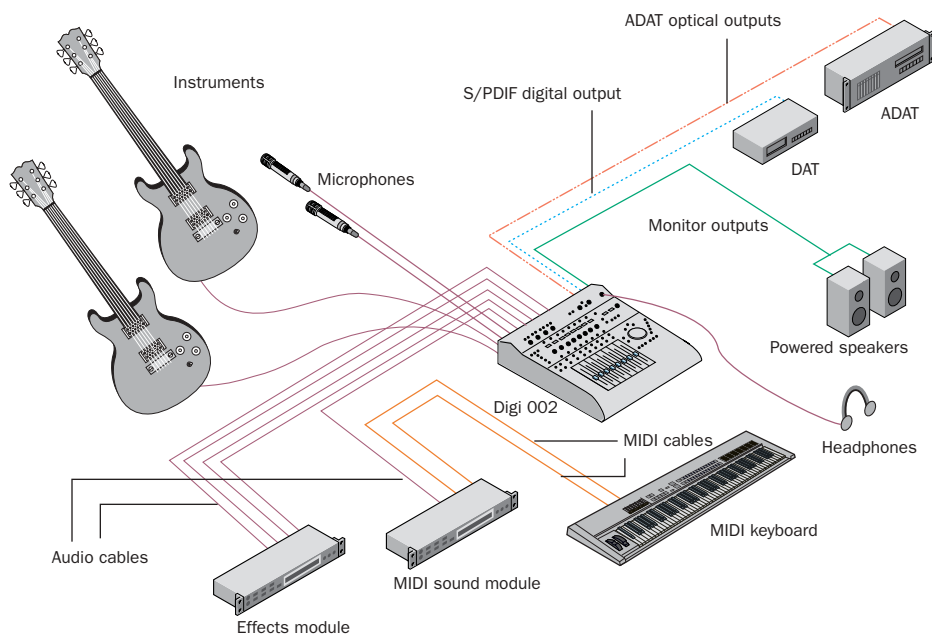
Figure 13. Digi 002 stand-alone studio configuration
