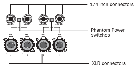
Mic/Line Inputs 1–4 (back panel)
