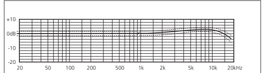
Frequency response curve BLM 3g, BLM 03Cg + CMC 6
