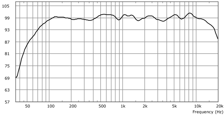
TCX-15 (dB) Sound pressure level
