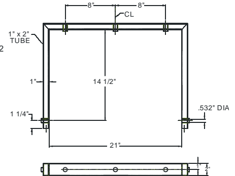
MOUNTING YOKE
