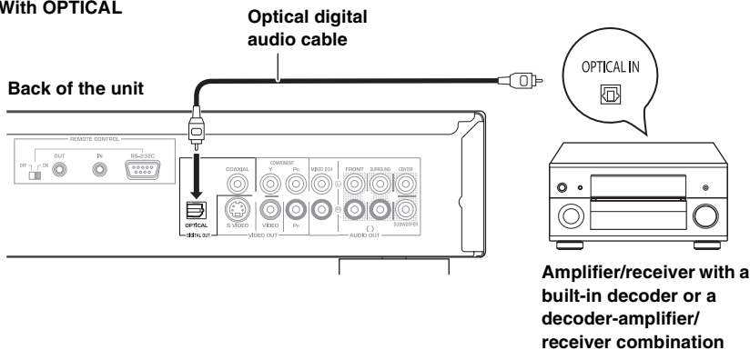
Amplifier/receiver with a built-in decoder or a decoder-amplifier/receiver combination
