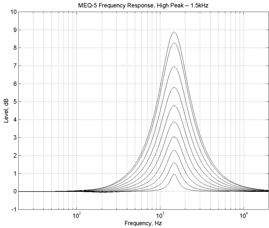
Figure 73. Pultec MEQ-5 High Peak Response
