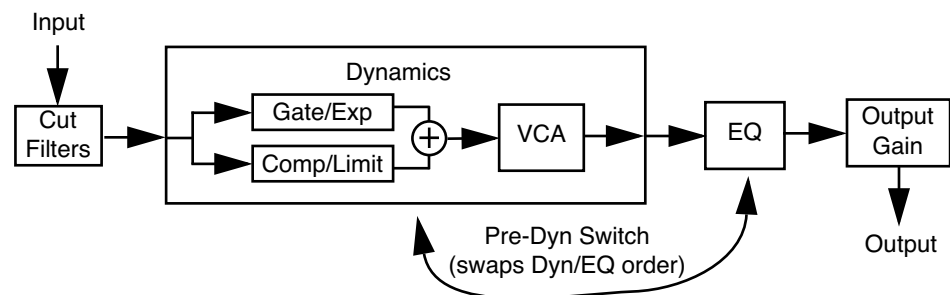
Figure 46. Simplified signal flow within UAD Neve 88RS
