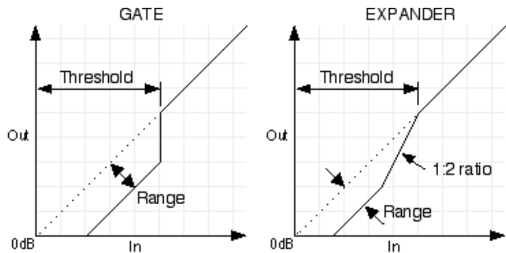
Figure 47. The Neve 88RS Gate/Expander diagram
