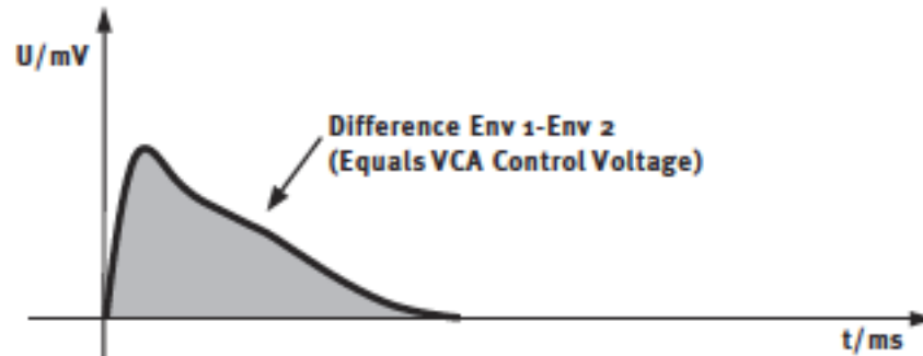
Figure 111. SPL Transient Designer Attack Control Voltage
