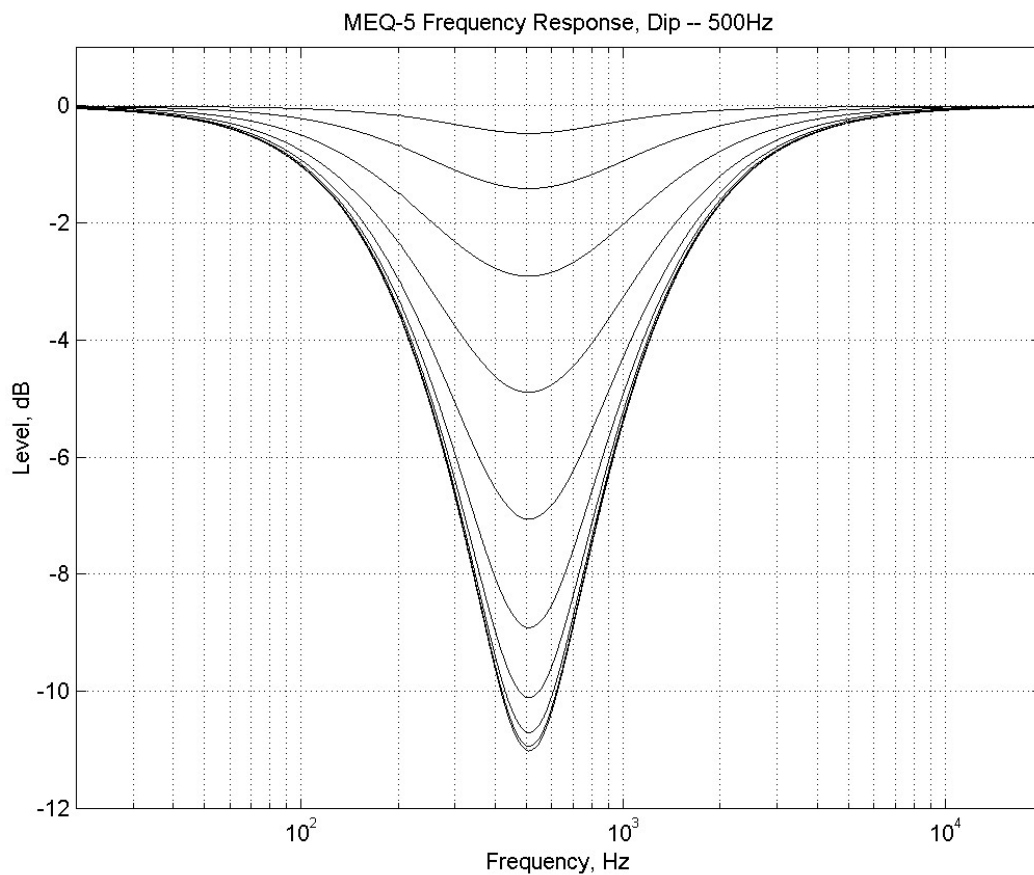
Figure 72. Pultec MEQ-5 Dip Response
