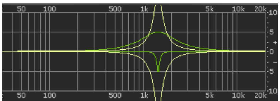
Figure 62. Parametric Type II response
