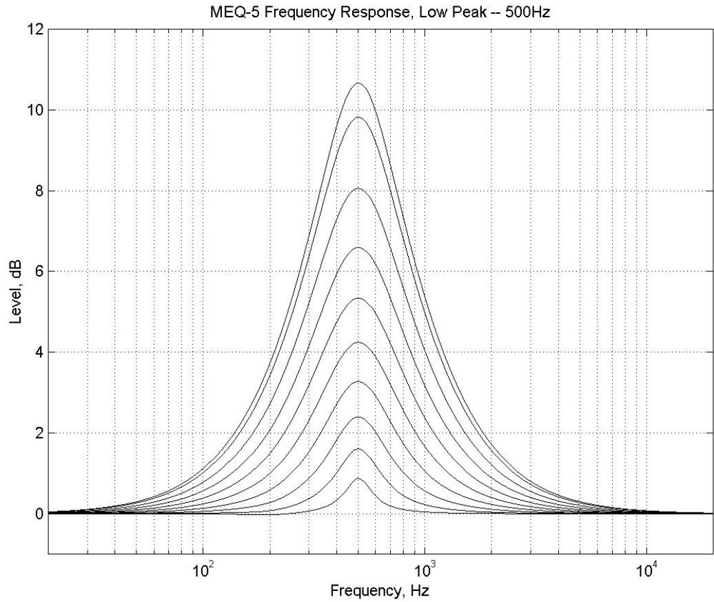
Figure 71. Pultec MEQ-5 Low Peak Response
