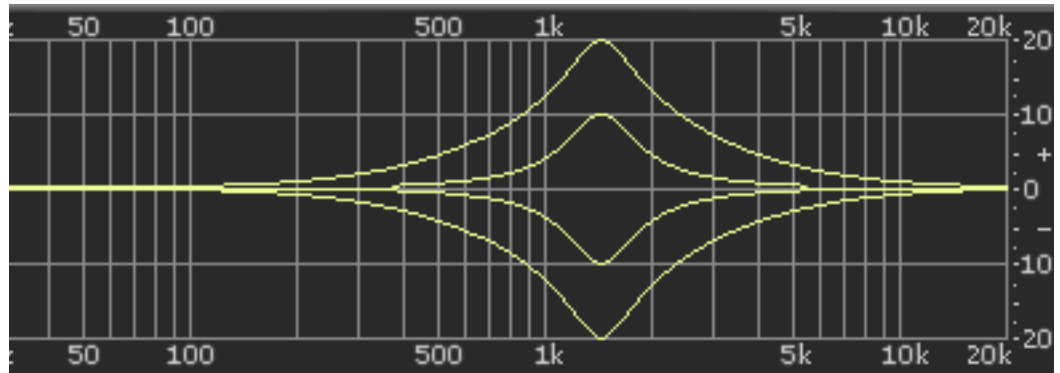
Figure 61. Parametric Type I response
