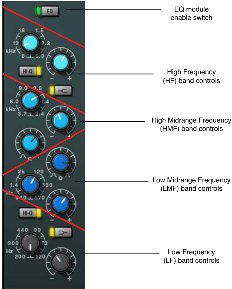
Figure 49. Neve 88RS EQ Controls Layout
