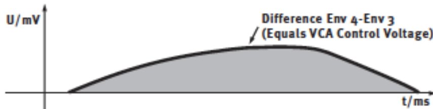
Figure 114. SPL Transient Designer Sustain Control Voltage
