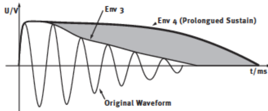
Figure 113. SPL Transient Designer Sustain Envelopes
