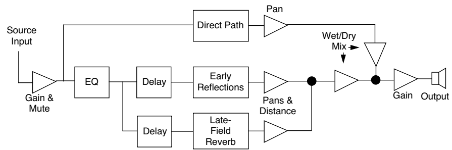
Figure 84. RealVerb Pro signal flow
