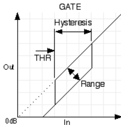
Figure 48. Hysteresis in the Neve 88RS Gate
