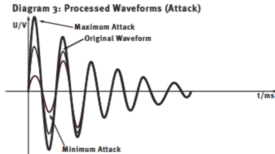
Figure 112. SPL Transient Designer Processed Attack
