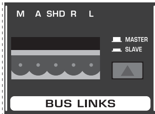
Fig. 4.3: Pin assignment of the BUS LINKS connector
