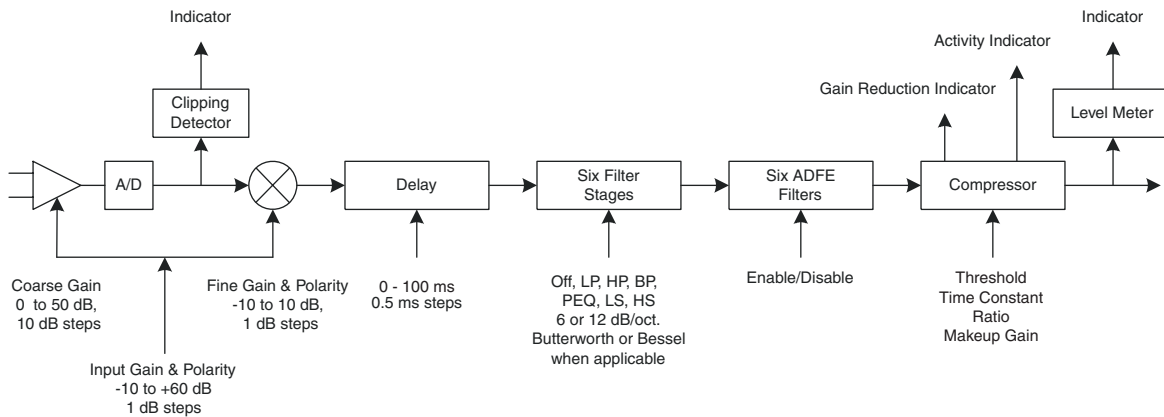
Typical Input Signal Processing Blocks
