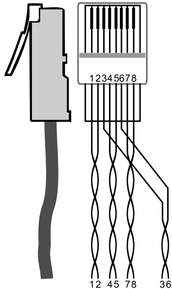
Figure 5: CAT 5 PINOUT
