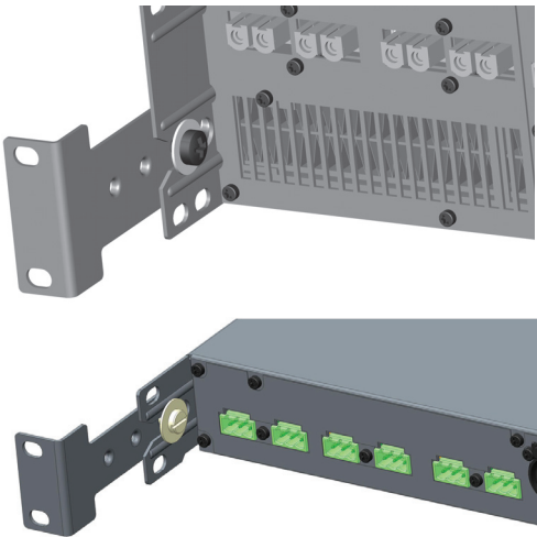
Rear support bracket mounted for fixed installation and bracket pointing forward
