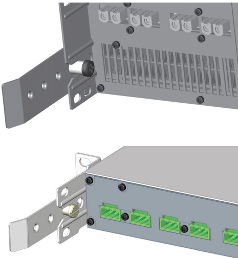
Rear support bracket mounted for removable installation and bracket pointing towards back
