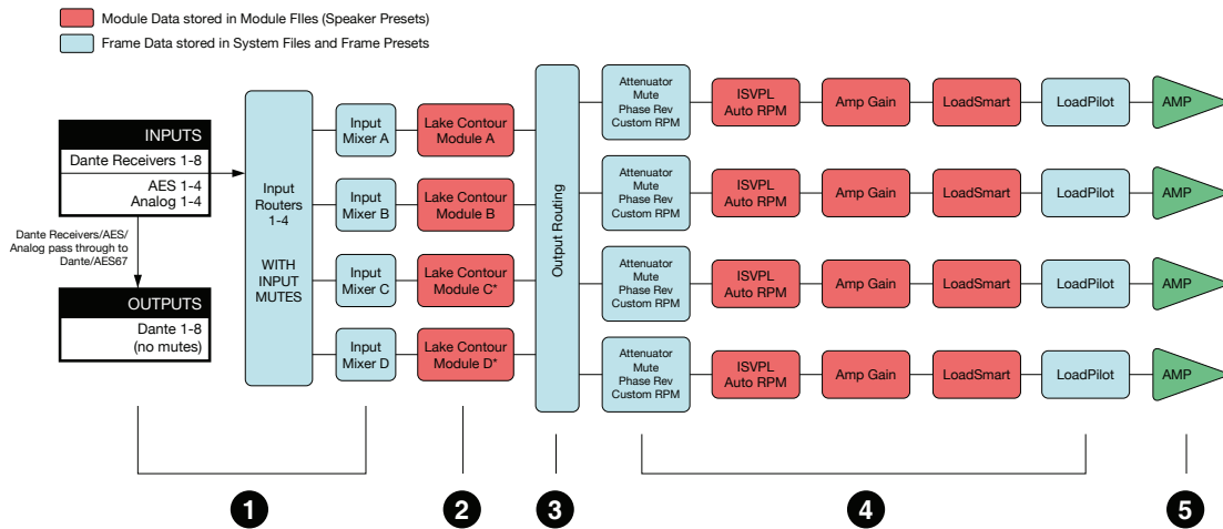
Figure 12.1: D Series Lake Signal Flow Diagram
