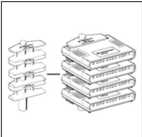
Radiator cluster with four IZK 20 clamps and IZM 20 cluster mounting kit
