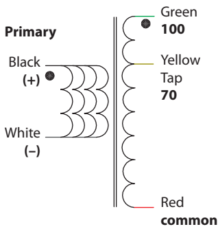
Figure 1. Schematic
