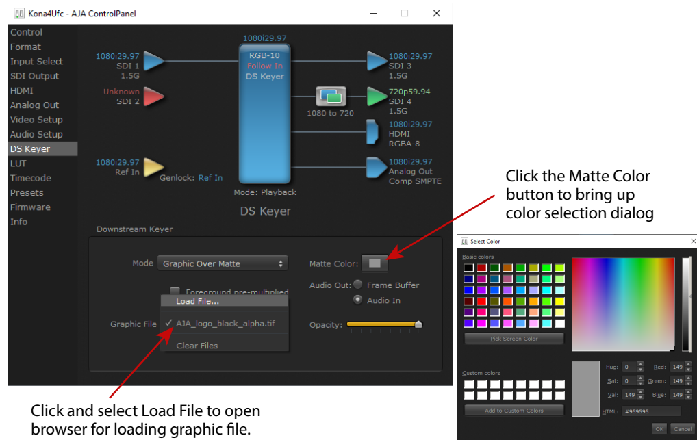
Figure 34. Graphic Selection and Matte Color Selection
