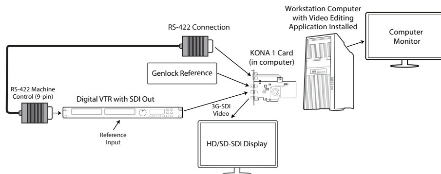
Figure 18. Typical KONA 1 System Connections
