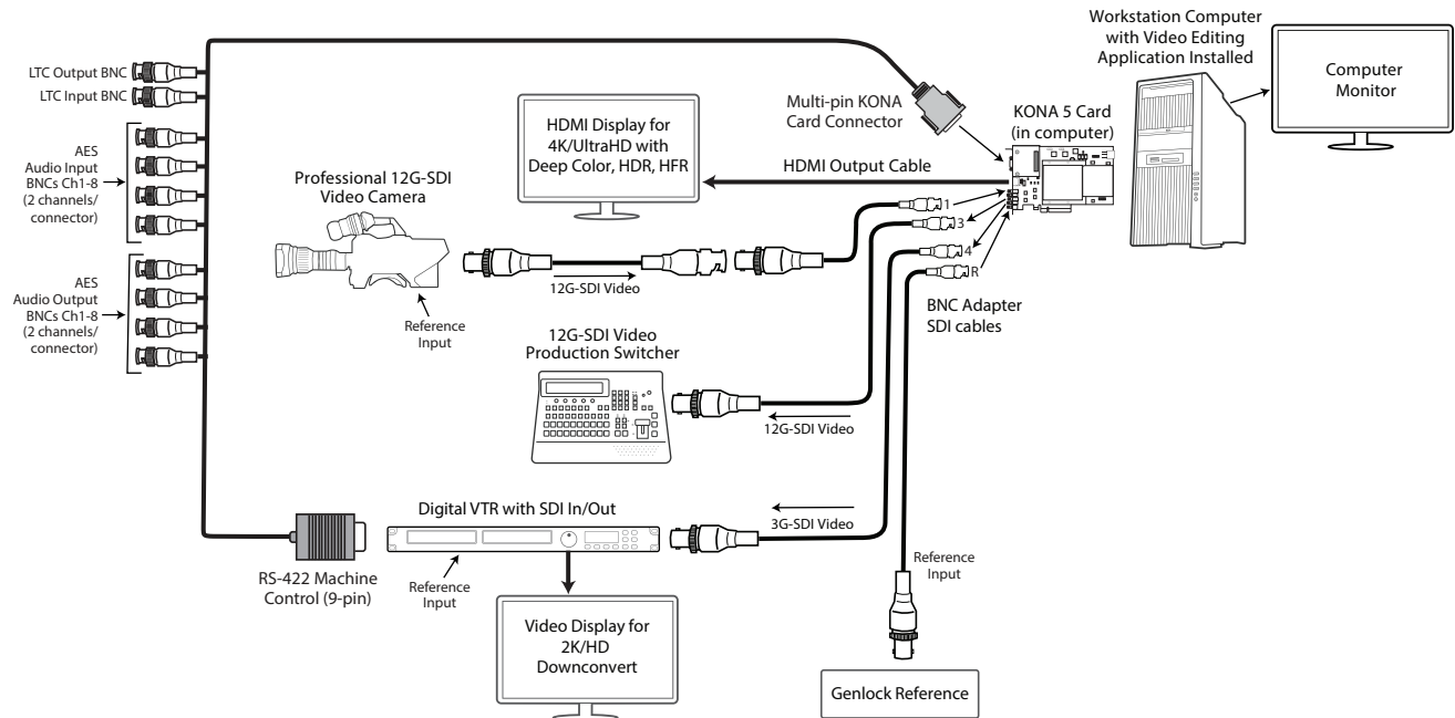
Figure 13. Typical KONA 5 System Connections, 4K Mode
