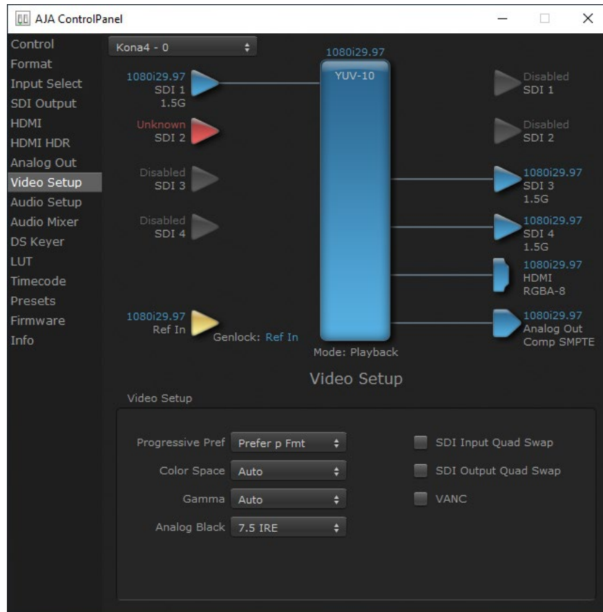
Figure 43. AJA Control Panel, Video Setup Screen
