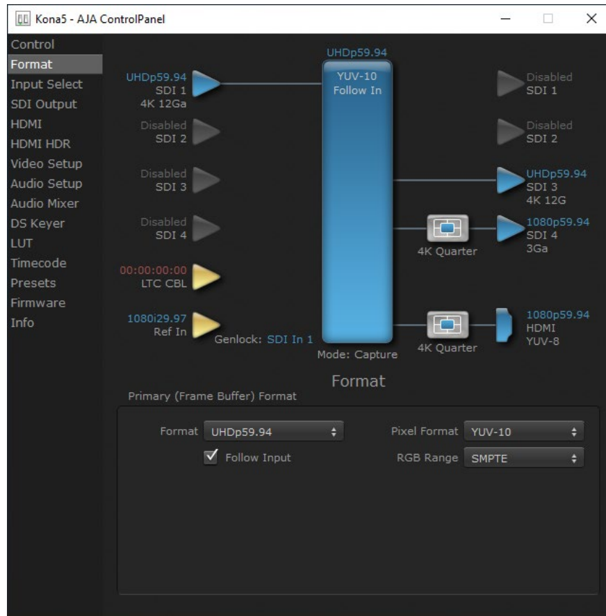
Figure 27. Format Screen, KONA 5
