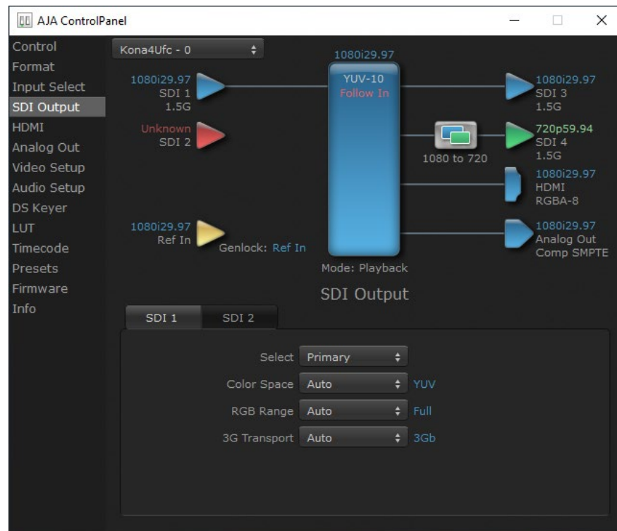
Figure 29. SDI Output Screen, KONA 4 in UFC Mode
