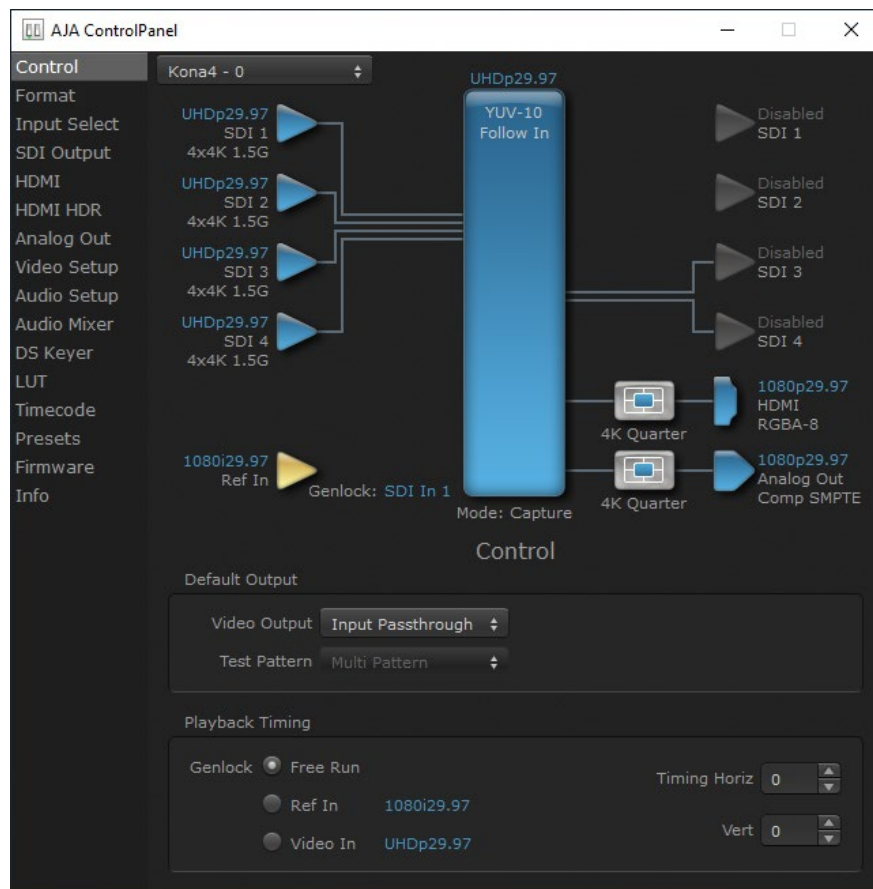
Figure 38. Control Screen with UltraHD 4 Link Input (KONA 4)
