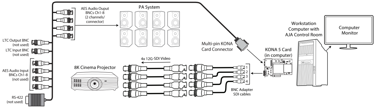
Figure 14. Typical KONA 5 System Connections, 8K Mode
