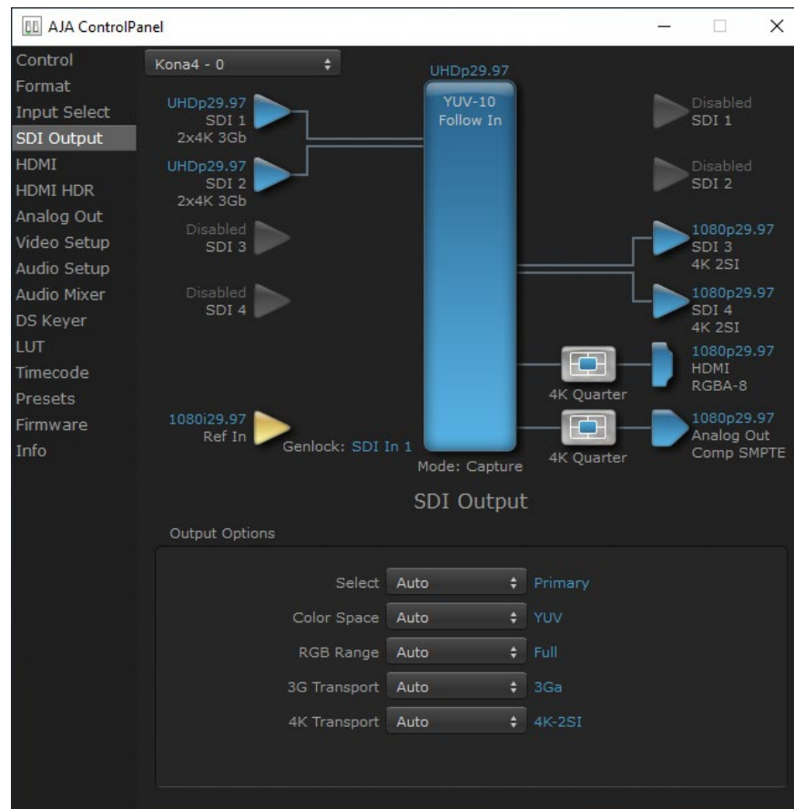
Figure 41. SDI Out Screen with 4K Format
