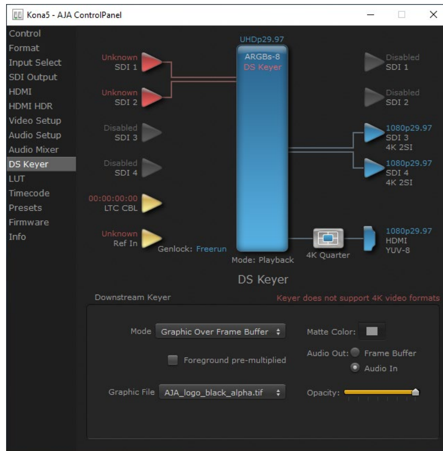
Figure 44. AJA Control Panel, DS Keyer Screen with Unsupported Message
