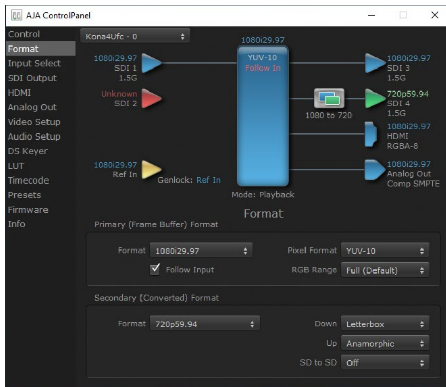
Figure 28. Format Screen, KONA 4 in UFC Mode
