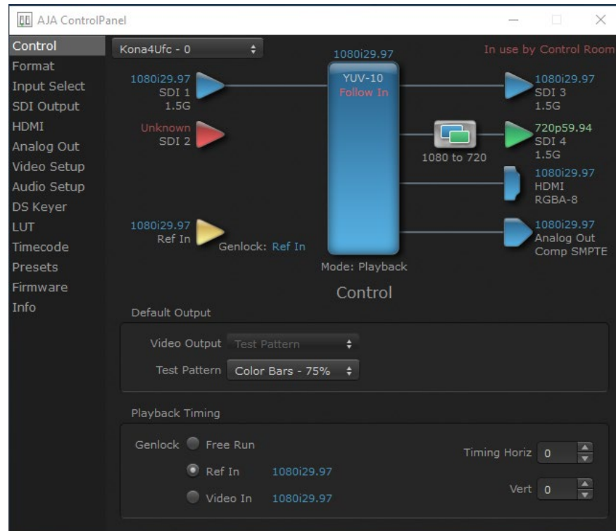
Figure 26. Control Screen, KONA 4 in UFC Mode
