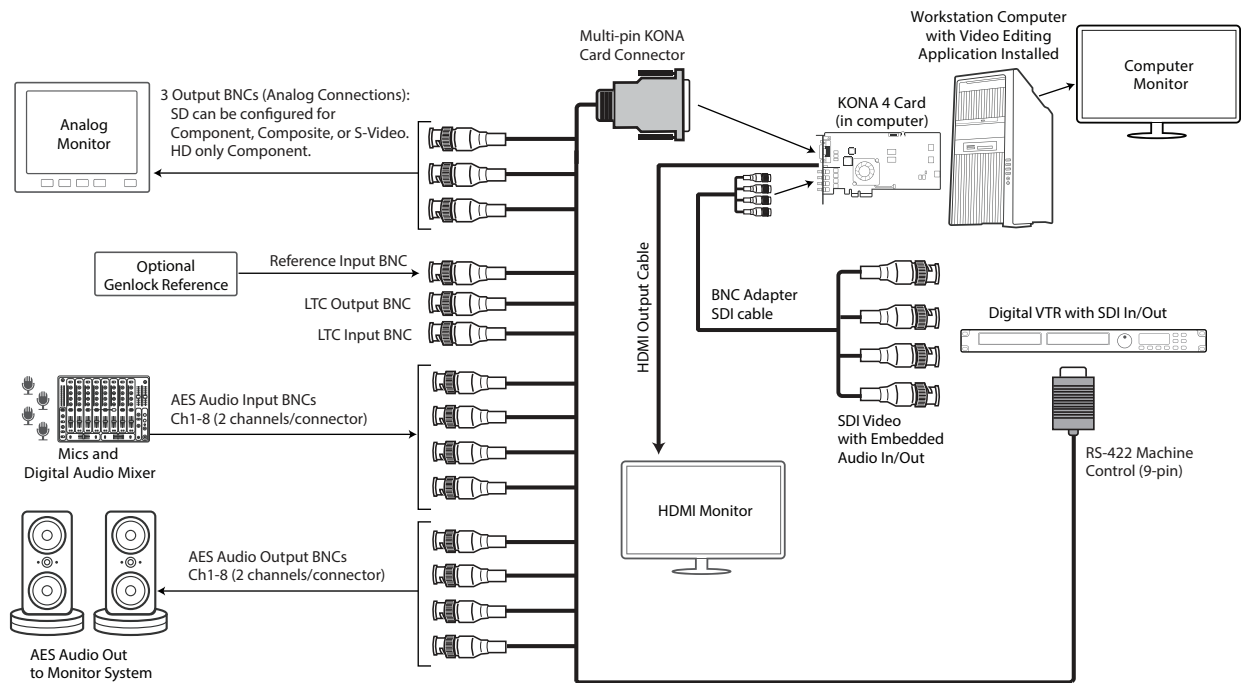
Figure 15. Typical KONA 4 System Connections
