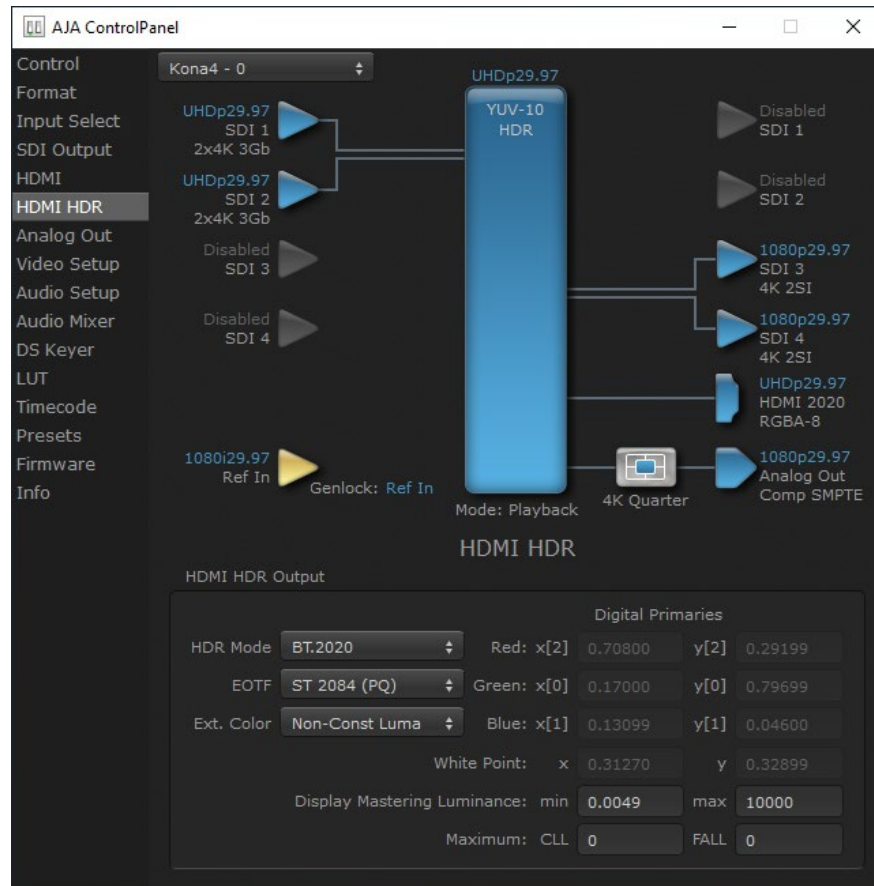
Figure 42. HDMI HDR Screen with 4K Primary Format
