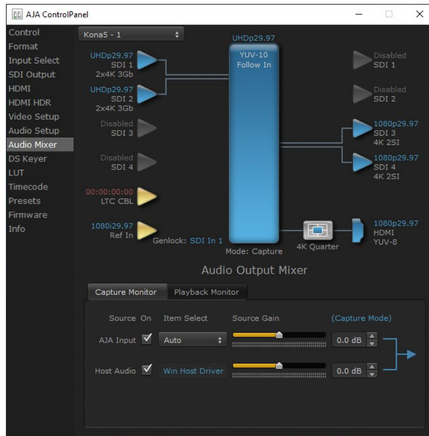
Figure 32. Audio Mixer Screen, Capture Monitor Mode, KONA 5
