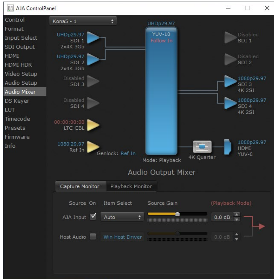
Figure 31. Audio Mixer Screen Example, KONA 5
