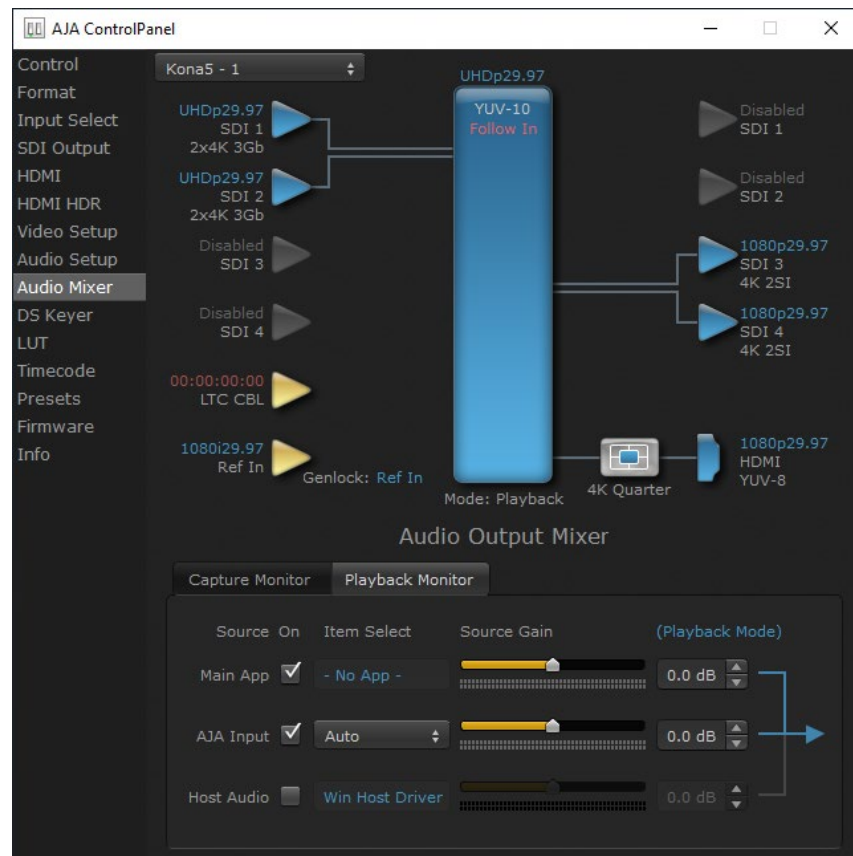
Figure 33. Audio Mixer Screen, Playback Monitor Mode, KONA 5
