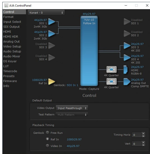
Figure 8. KONA 4 AJA Control Panel Screen Example
