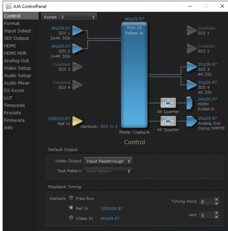
Figure 39. Control Screen with 4K 2 Link Input and Output (KONA 4)
