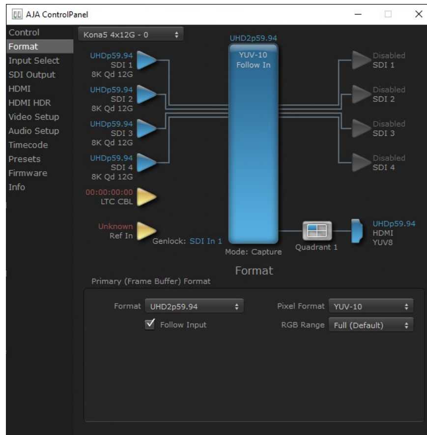
Figure 45. AJA Control Panel, KONA 5 Format Screen in 8K Mode
