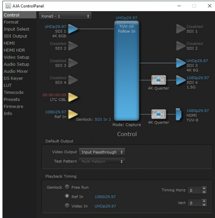
Figure 40. Control Screen with UltraHD and HD Output (KONA 5)
