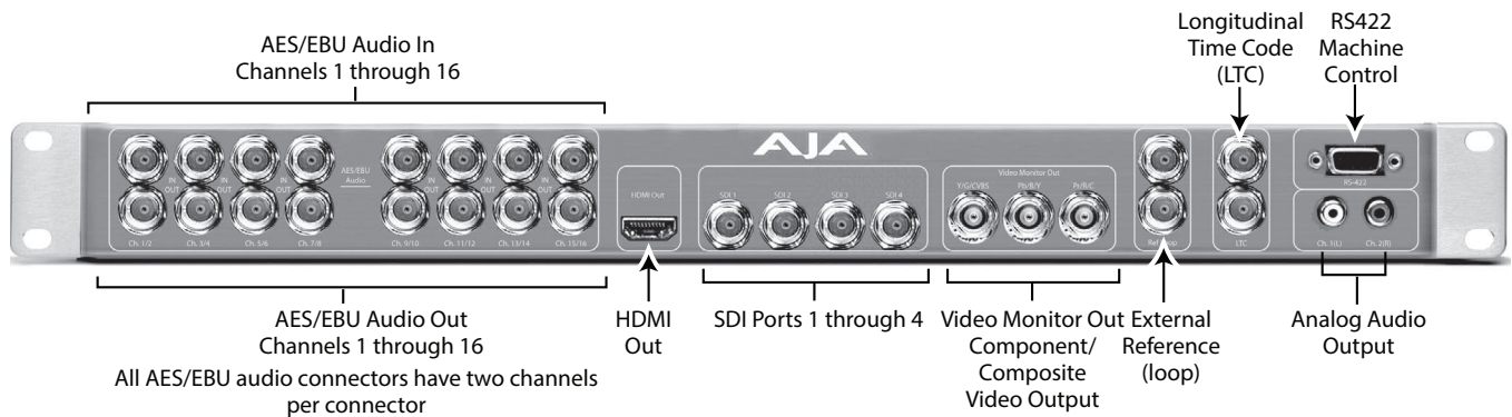
Figure 17. K3G-Box Model Breakout Box (rear view)
