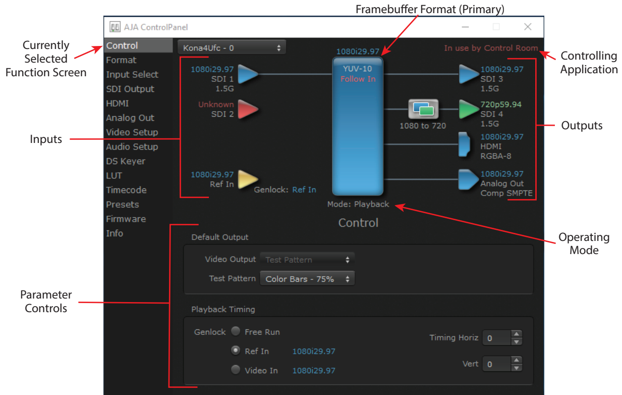
Figure 20. AJA Control Panel, Block Diagram and Controls
