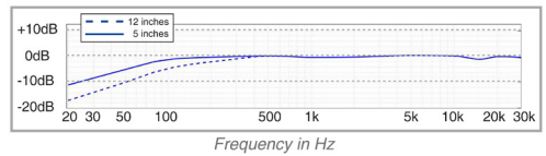
Frequency Response of P30/C (typical)
