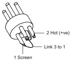
XLR Unbalanced input
