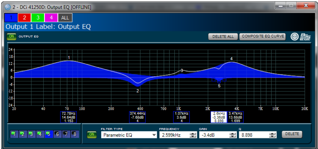
Figure 43: EQ panel
