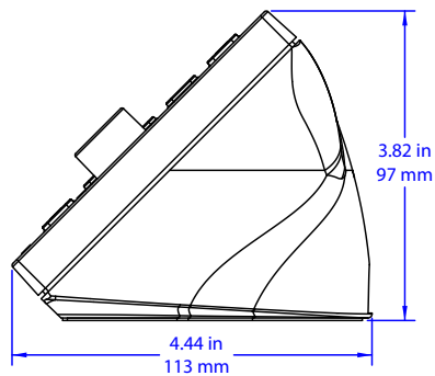
TTK with MPC3-302 Device Installed
