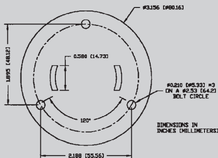
Mounting Flange Detail
