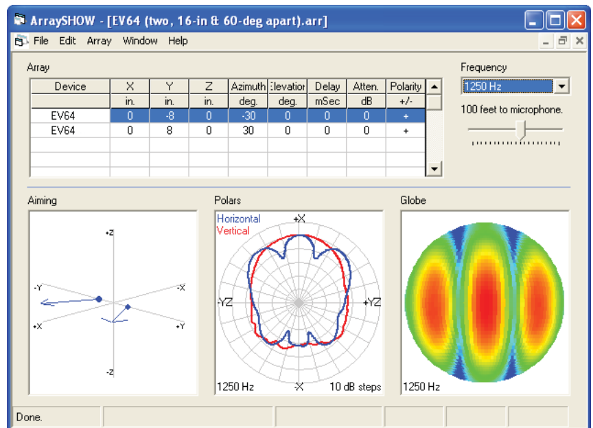
Figure 6: Horizontal polar response (blue center plot) of two closely clustered 60° x 40° loudspeakers aimed 60° apart, showing the off-axis nulls at 1,250 Hz caused by multiple-source interference (see text for more details)
