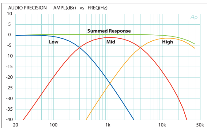
Three Program EQ filter bands and the flat summed response
