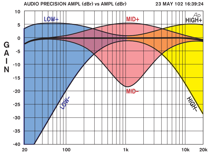
Interactivity of the Accelerated-Slope™ EQ controls
