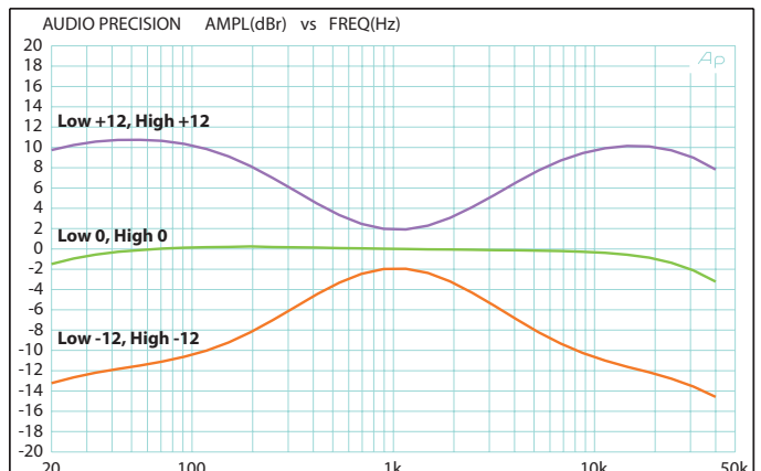
Combined response of the Mic and Headphone Tone controls
