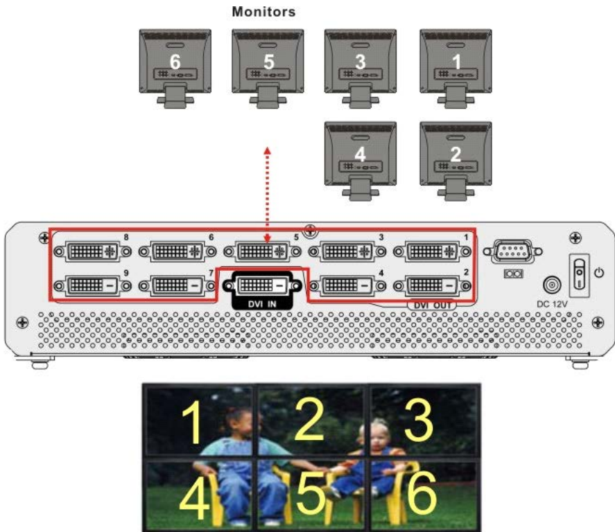
Figure 20. 3 x 2 array for VWL-B133FD
