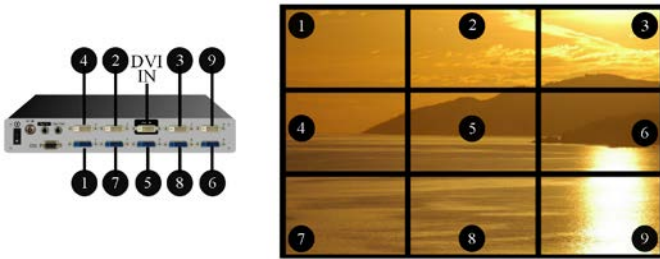
Figure 6. 3 x 3 Installation
