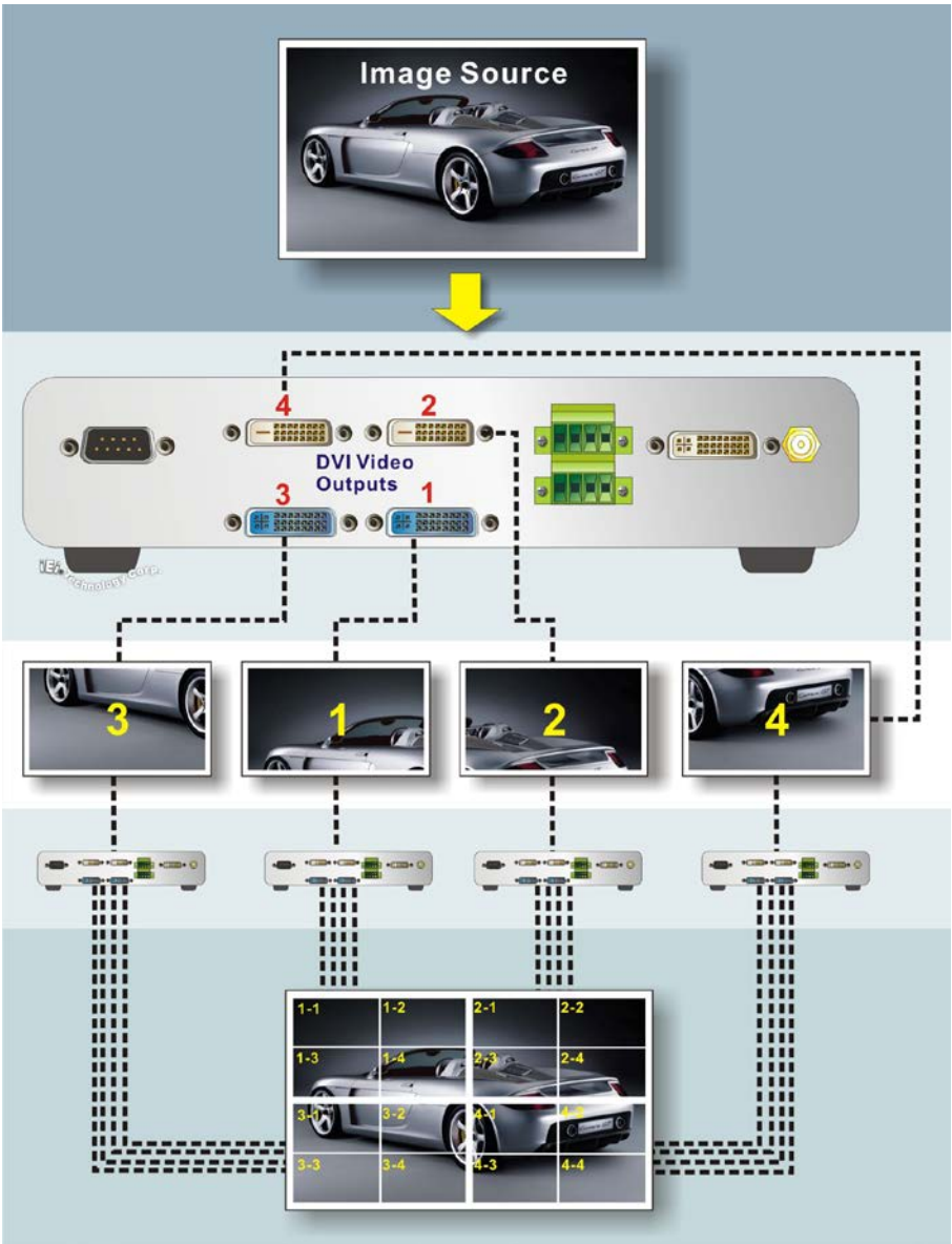
Figure 17. 4 x 4 array for VWL-B122FD
