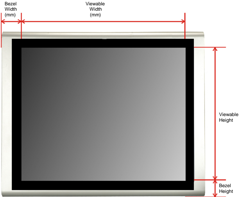
Figure 7. Bezel calculation for VWL-B133FD
