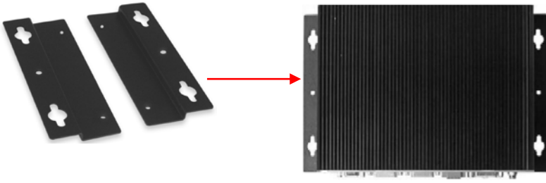
Figure 9. Mounting Brackets
