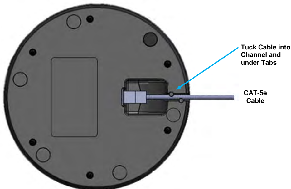
Diagram: EasyMic MicPOD Installation Diagram (bottom view)
