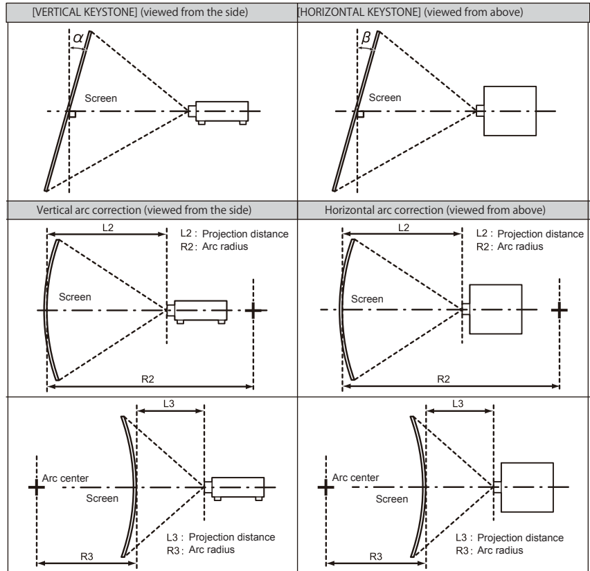
When Vertical keystone and Horizontal keystone are used simultaneously, correction cannot be made exceeding total of 55°
