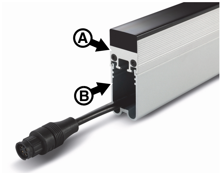
Figure 3: Mounting profile: end view
