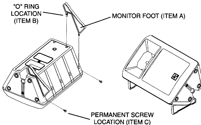
FIGURE 1 — Installing the F200 Monitor Foot on System 200™ Speaker
