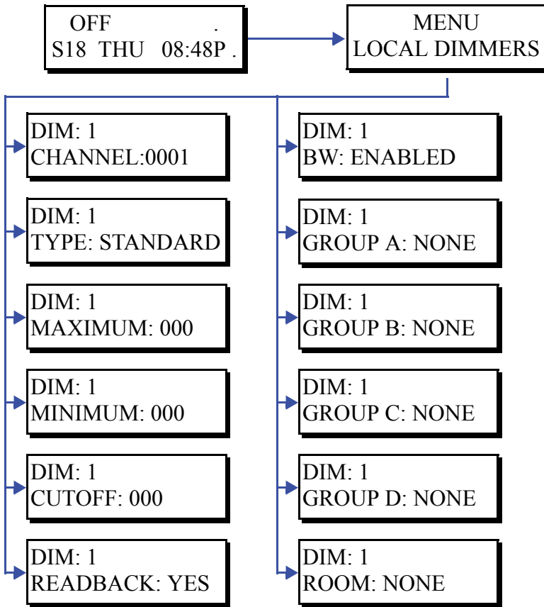
Dimmer Configuration Menu Chart
