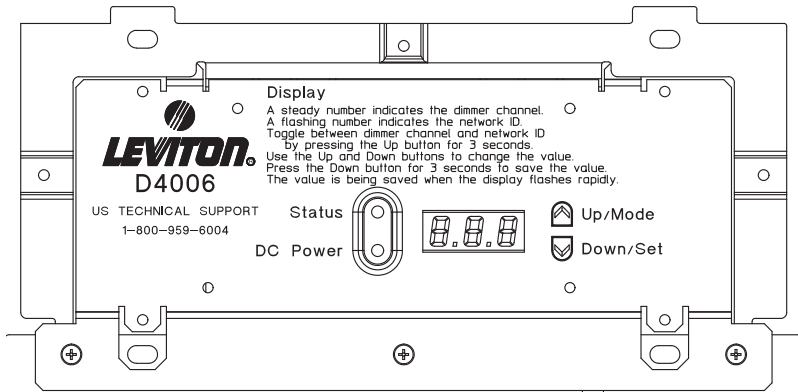
D4006 - Front Panel
