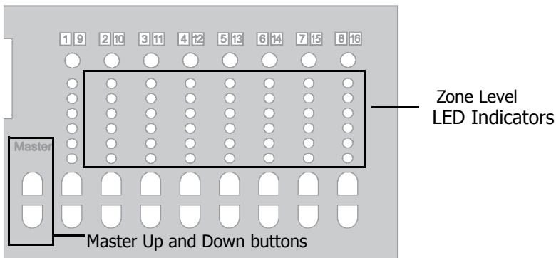
Figure 17 - Zone Level Indicators
